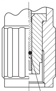
RSMA CONNECTOR DETAILS
